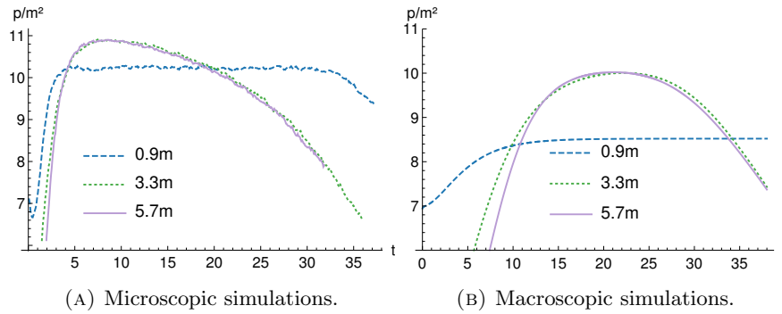
FIGURE 12. Simulations for n = 60 , \beta = 3.84 , \mu = 1 . We observe a good agreement between the CA (microscopic) and PDE (macroscopic) solutions. The effect of higher densities for wider corridors also occur on a macroscopic scale. There is a clear difference in behavior between narrow and wide corridors
