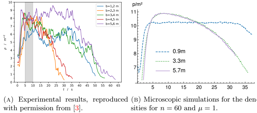
FIGURE 7. Impact of the corridor width on the maximum density. The CA approach yields comparable results for high density regimes and low motivation level.
